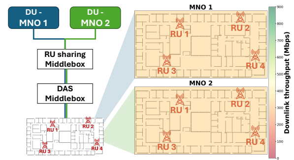
Figure 12: Chaining of RU sharing and DAS middlebox to enable multi-tenancy with seamless coverage.
