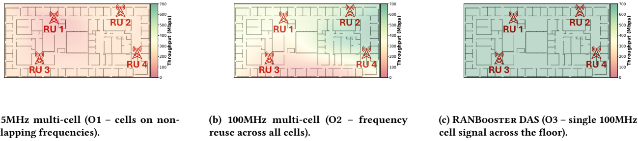
Figure 11: Performance of simple 4 RU RANBooster DAS deployment vs multi-cell deployment configurations.
